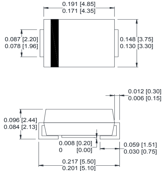
SMB/ DO-214AA
