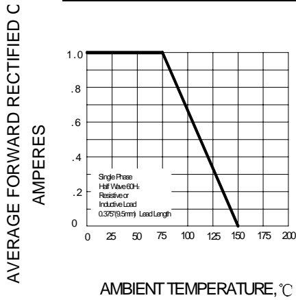
FIG.1 – FORWARD DERATING CURVE
