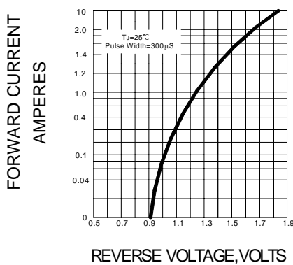
FIG.3-TYPICAL FORWARD CHARACTERISTIC
