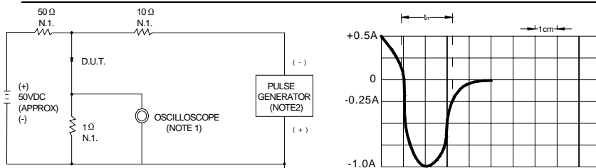
FIG.6 – REVERSE RECOVERY TIME CHARACTERISTIC AND TEST CIRCUIT DIAGRAM
