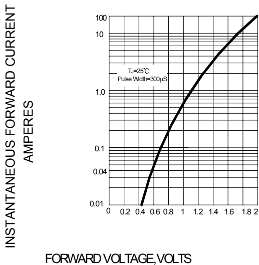
FIG.4–TYPICAL FORWARD CHARACTERISTICS
