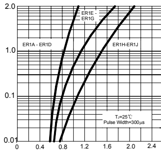
FIG.2 – TYPICAL FORWARD CHARACTERISTIC
