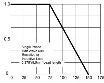
FIG.3 – FORWARD DERATING CURVE
