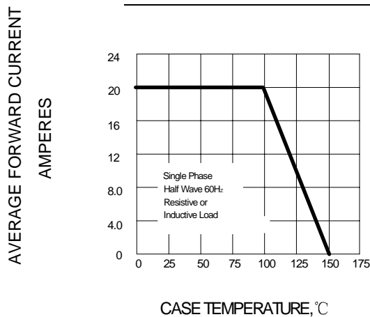
FIG.4-FORWORD DERATING CURVE
