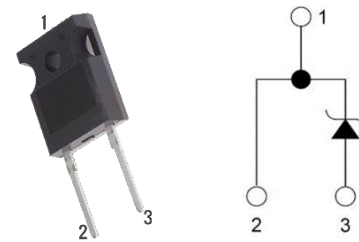
TO-247-2
