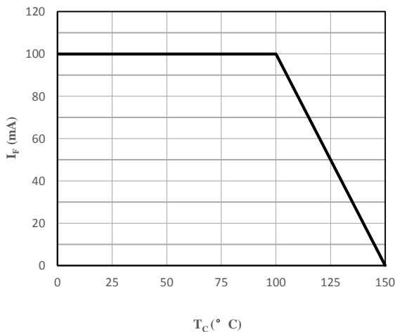
Fig 5 Current Derating
