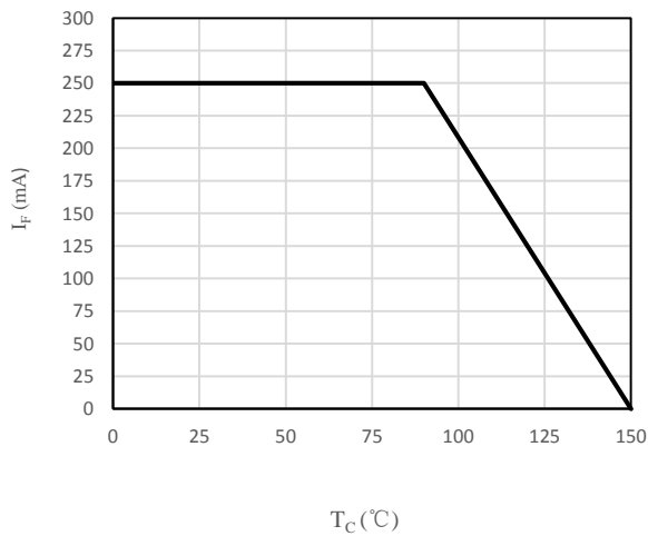
Fig 3 Current Derating Curve
