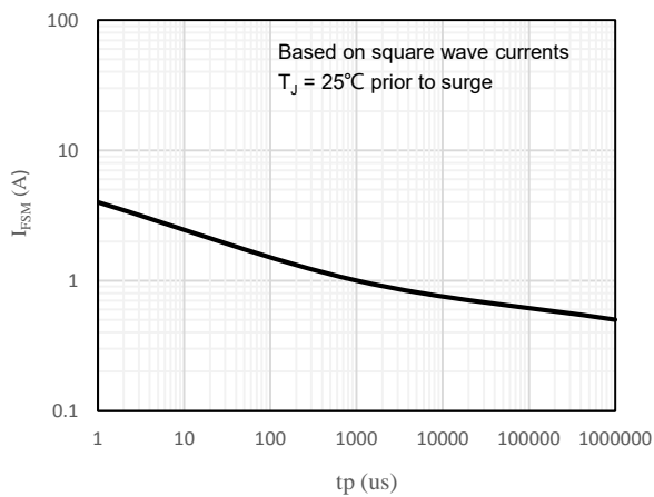
Fig 5 Non-repetitive peak forward current as a function of pulse duration; maximum values
