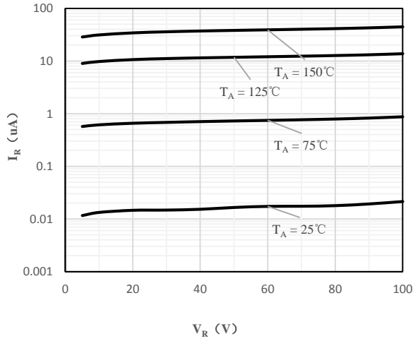
Fig 1 Typical Reverse Characteristic
