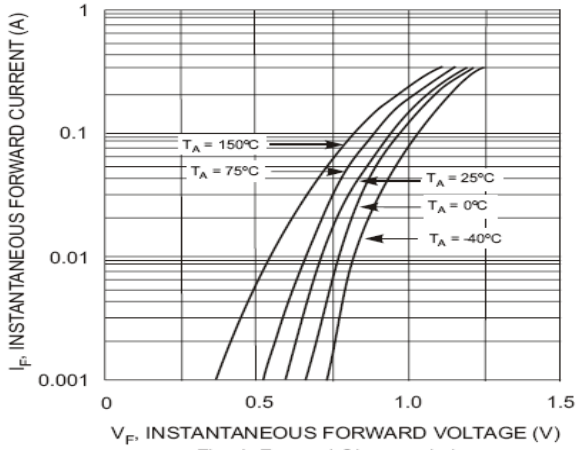
Fig. 1 Forward Characteristics
