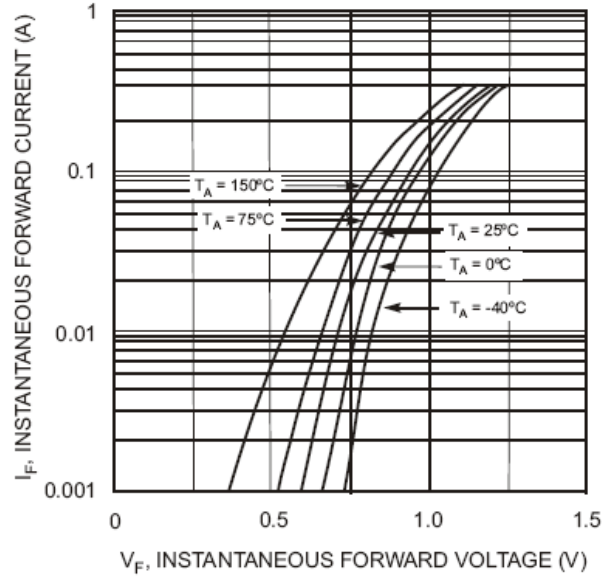
Fig. 2 Forward Characteristics
