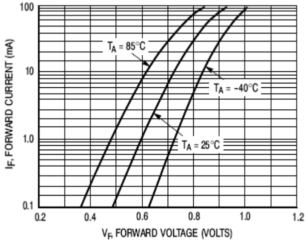
Figure 2. Forward Voltage
