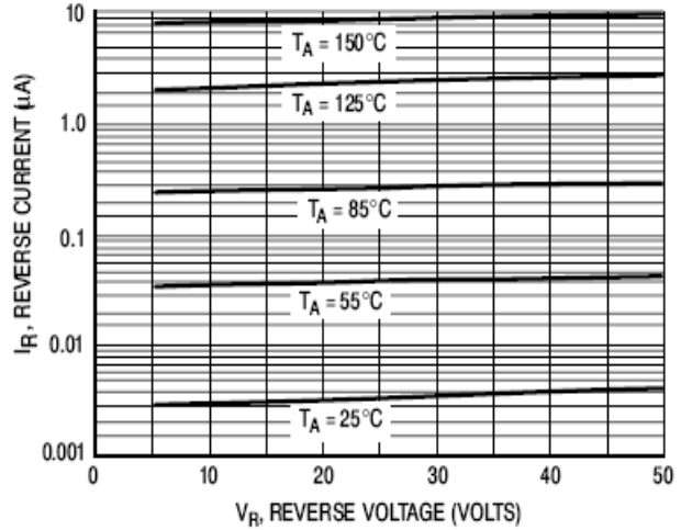
Figure 3. Leakage Current
