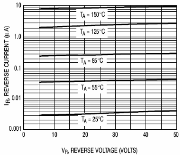
Figure 2. Leakage Current
