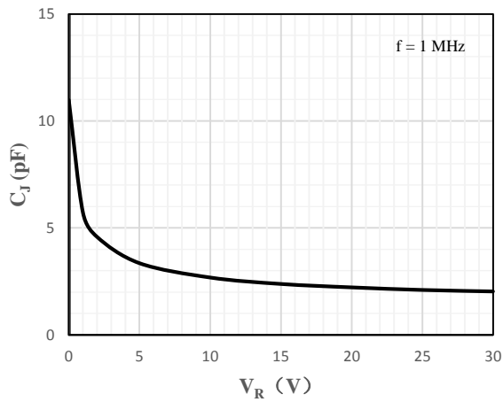
Fig 3 Capacitance Characteristics
