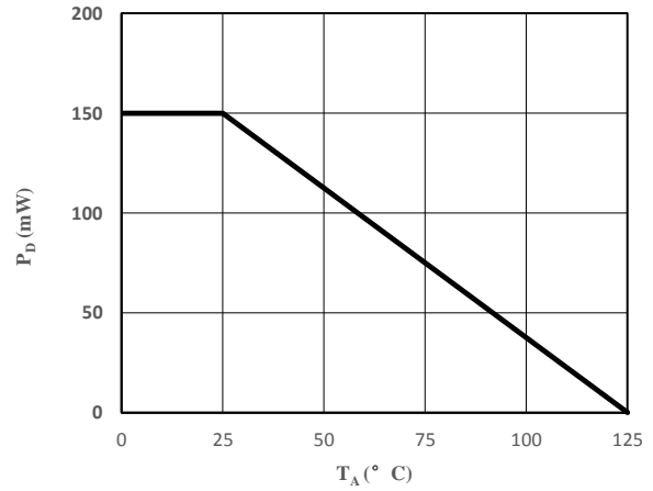
Fig 4 Derating Curve
