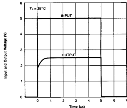
Figure 6. Pulse Response
