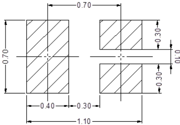
DFN1006-3
