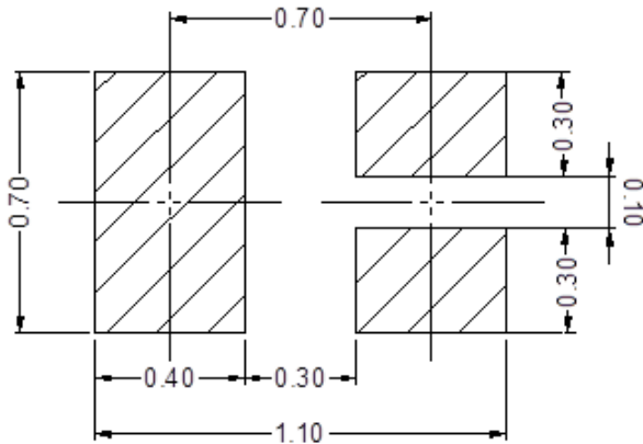
DFN1006-3
