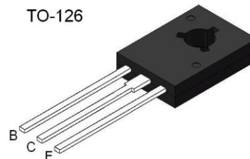
TO-126
