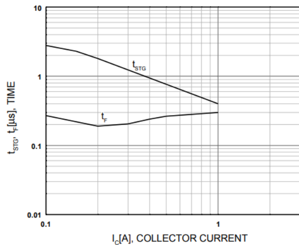
Figure 4. Switching Time
