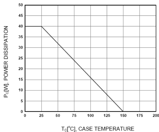
Figure 4. Power Derating
