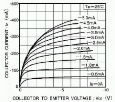
Fig.3 Grounded emitter output characteristics ( II )
