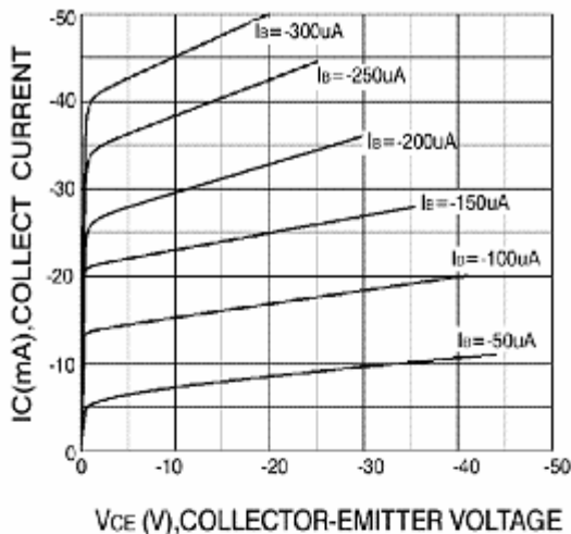
Static Characteristic
