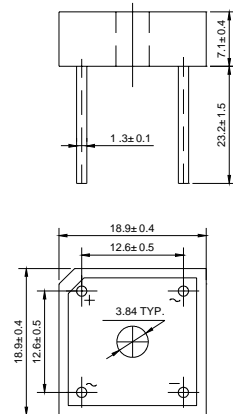
Dimensions in millimeters
