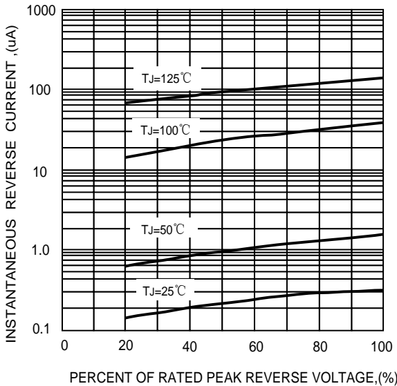
FIG.3-TYPICAL REVERSE CHARACTERISTICS
