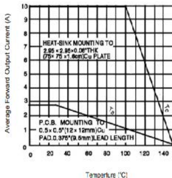
Figure 2. Forward Output Current Derating Curve
