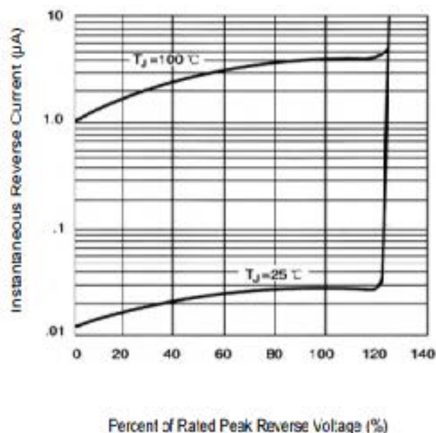
Figure 4. Typical Reverse Characteristics Per Element
