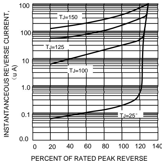
FIG.5-TYPICAL REVERSE
