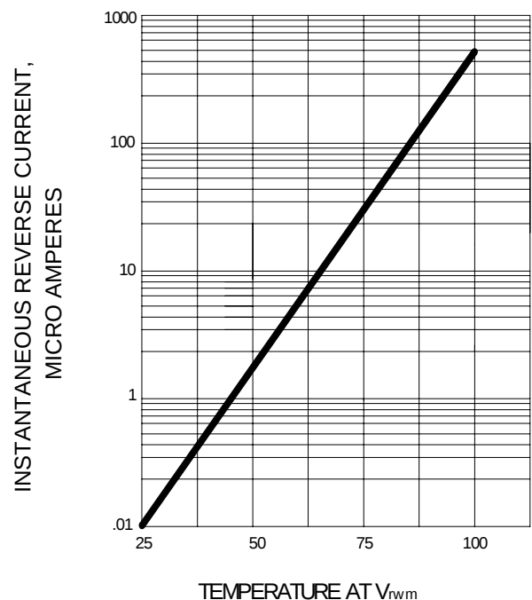
FIG.3-- TYPICAL REVERSE CHARACTERISTIC
