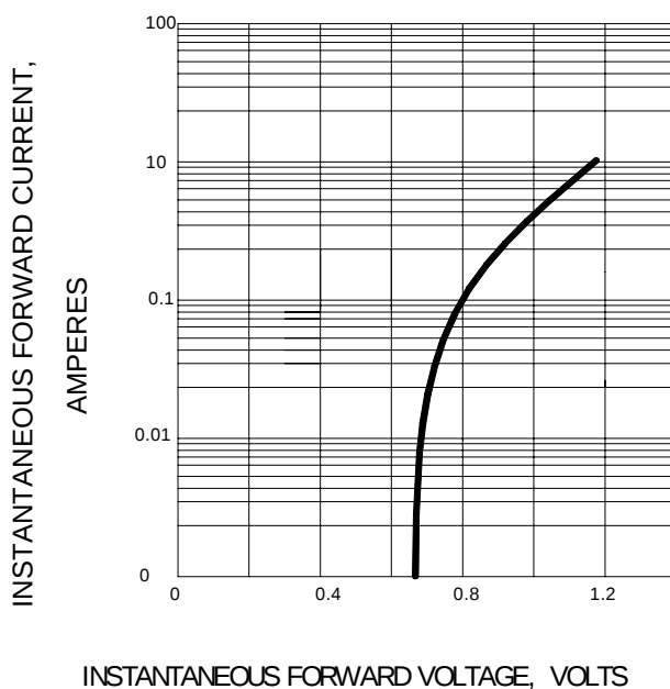
FIG.2 -- TYPICAL FORWARD CHARACTERISTIC
