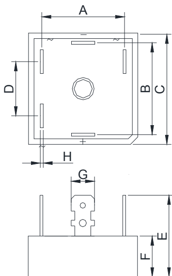
SKBPC
