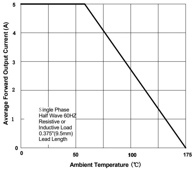
FIG.1: Io-Ta Curve
