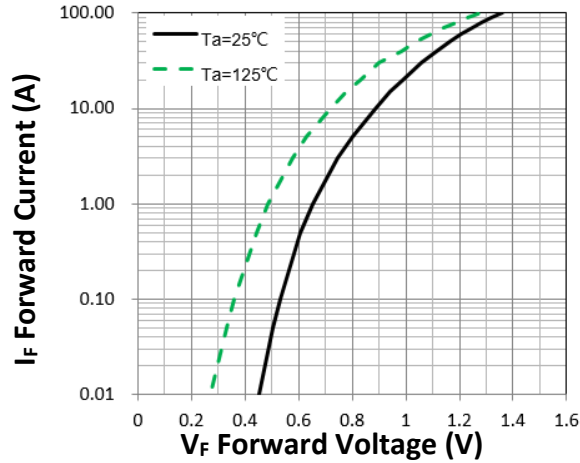
Figure 1. Forward Characteristic(typ.)
